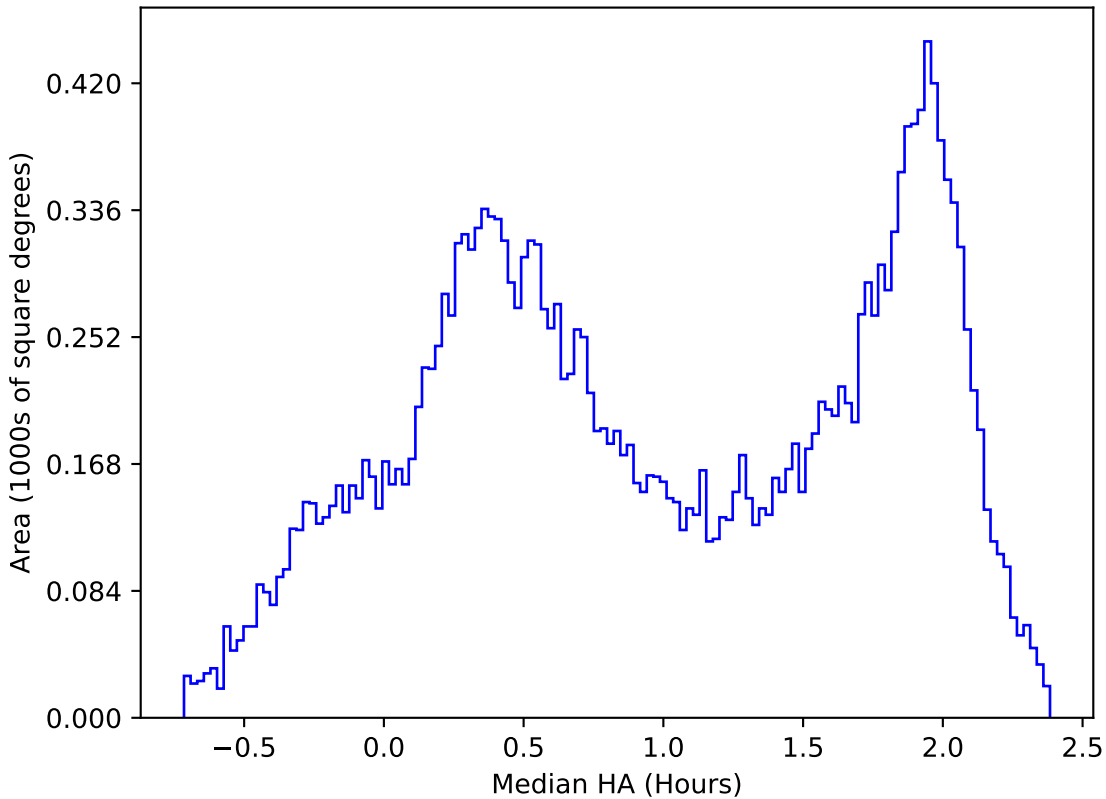
noroll_mjdp365_v3.4_10yrs All sky y band: Median HA
