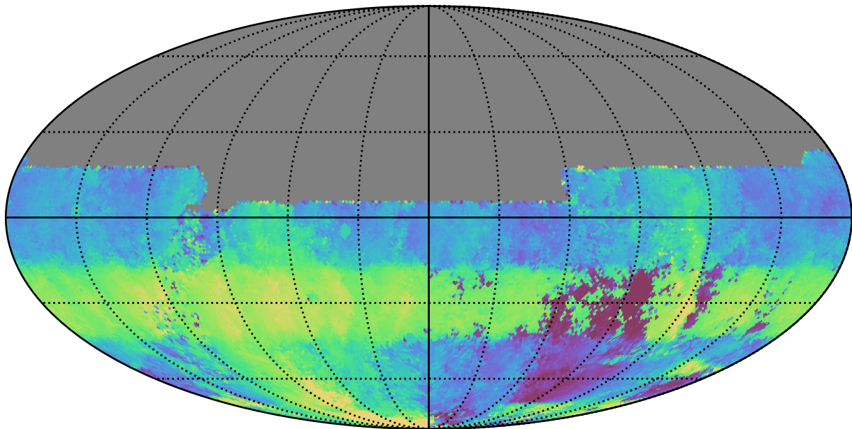
noroll_mjdp365_v3.4_10yrs All sky u band: Median HA
