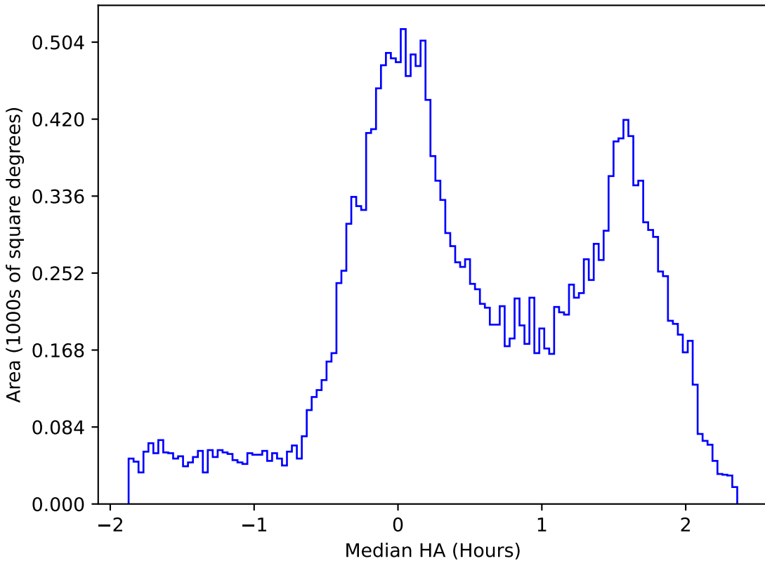
noroll_mjdp365_v3.4_10yrs All sky u band: Median HA
