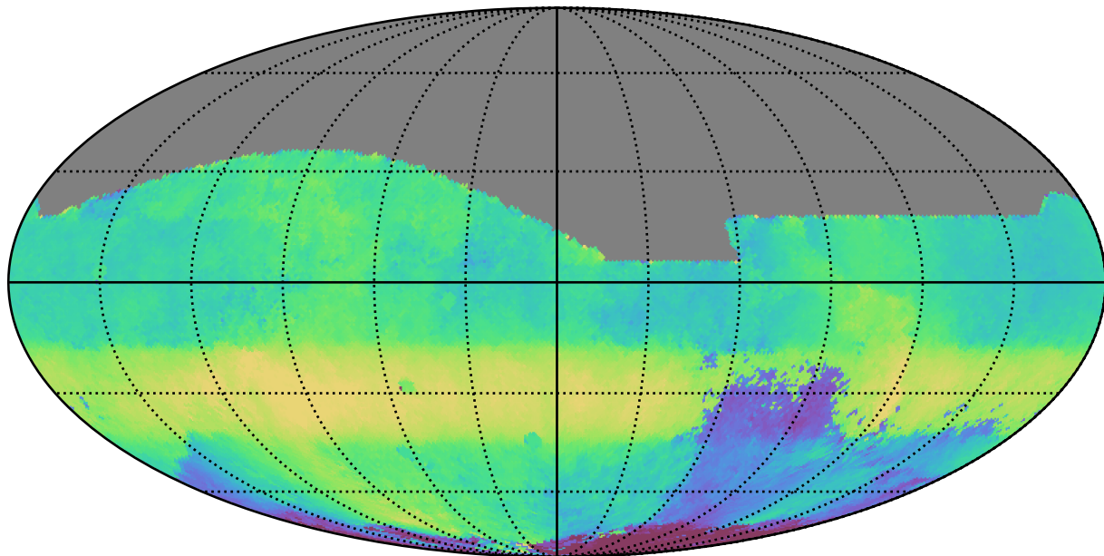
noroll_mjdp365_v3.4_10yrs All sky r band: Median HA
