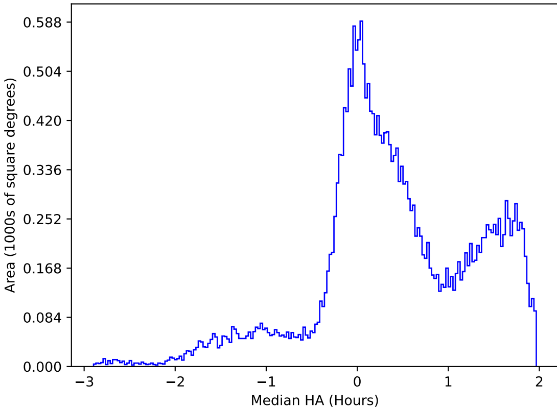
noroll_mjdp365_v3.4_10yrs All sky r band: Median HA
