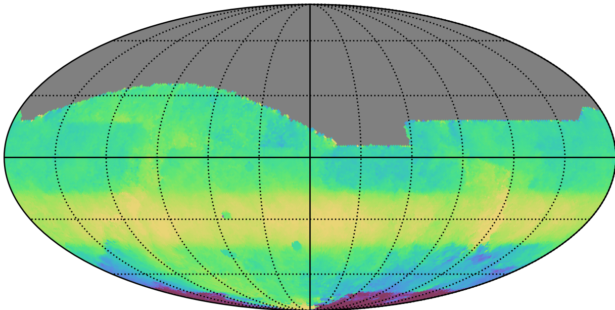
noroll_mjdp365_v3.4_10yrs All sky i band: Median HA
