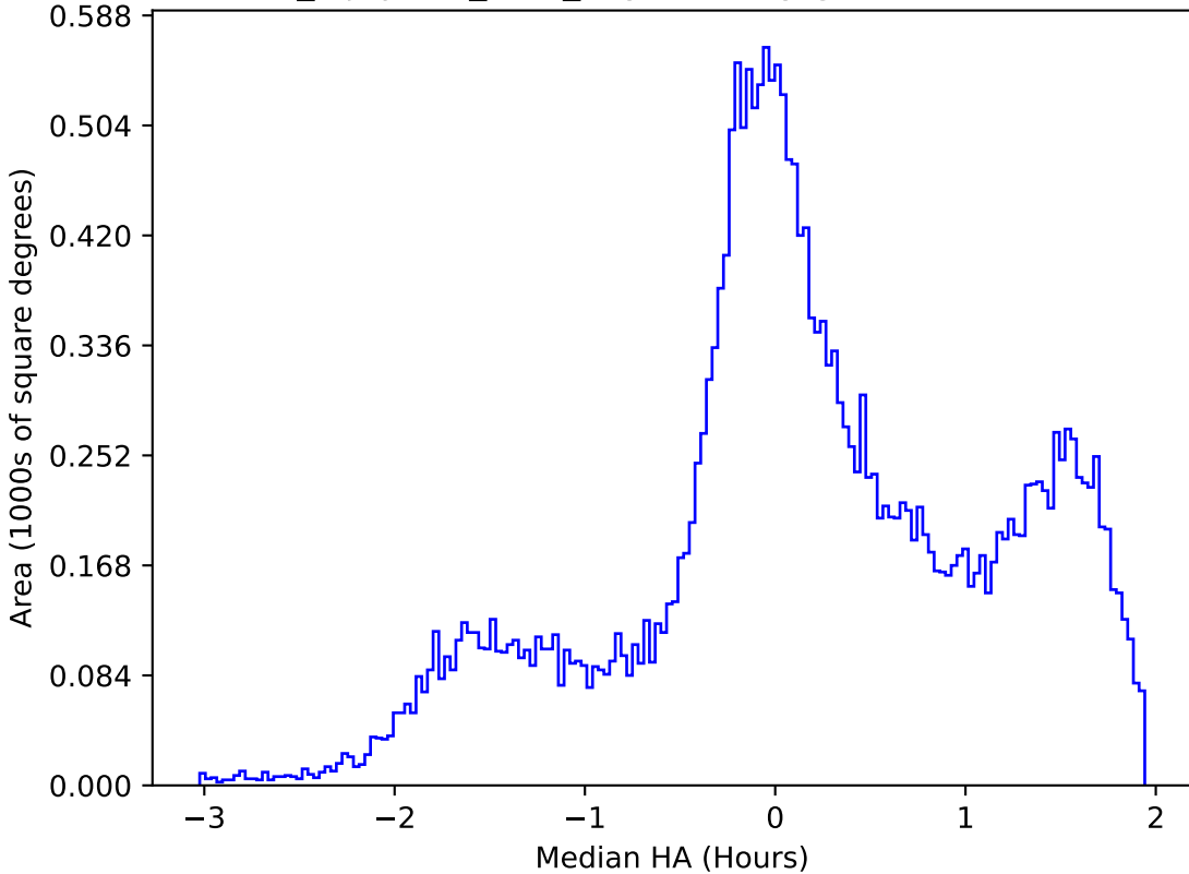
noroll_mjdp365_v3.4_10yrs All sky g band: Median HA
