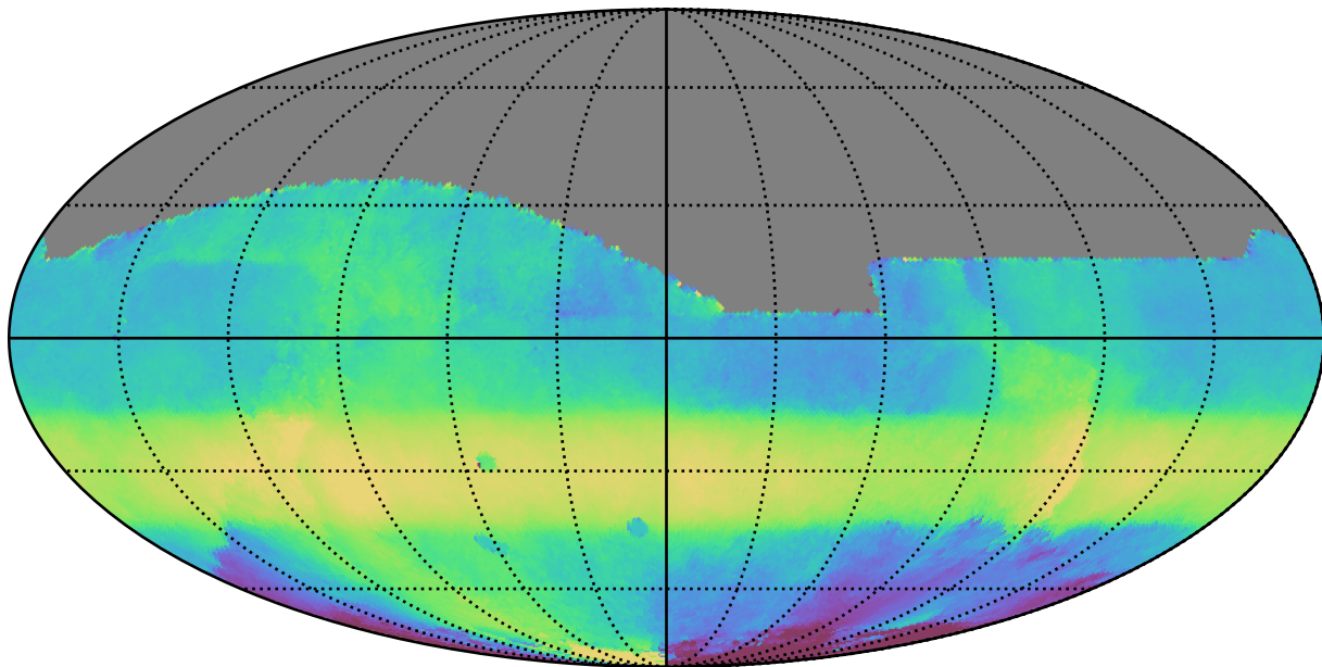
noroll_mjdp365_v3.4_10yrs All sky all bands: Median HA
