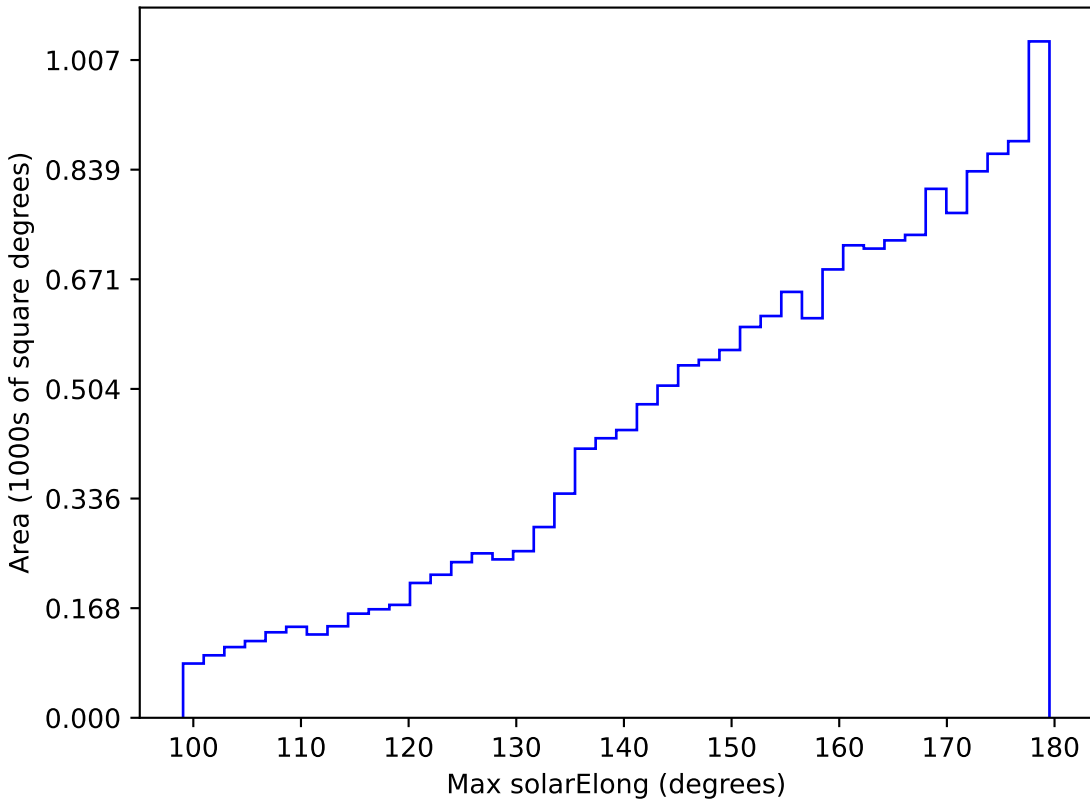
noroll_mjdp365_v3.4_10yrs WFD r band: Max solarElong
