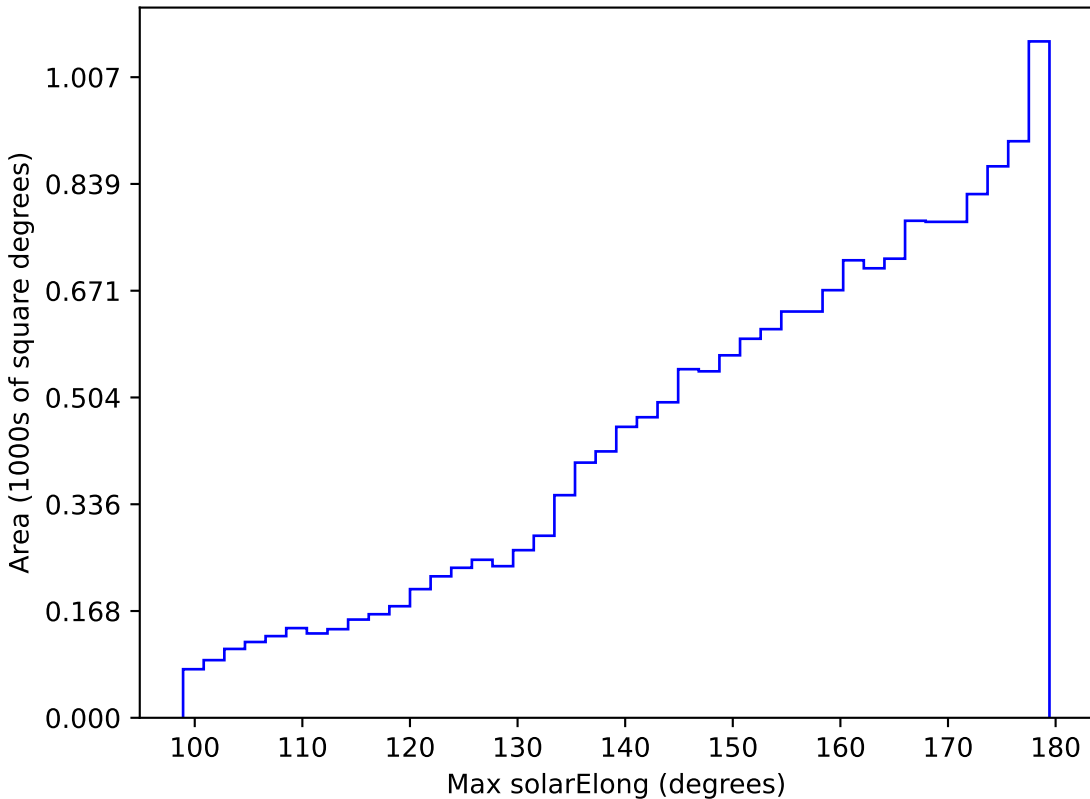
noroll_mjdp365_v3.4_10yrs WFD i band: Max solarElong
