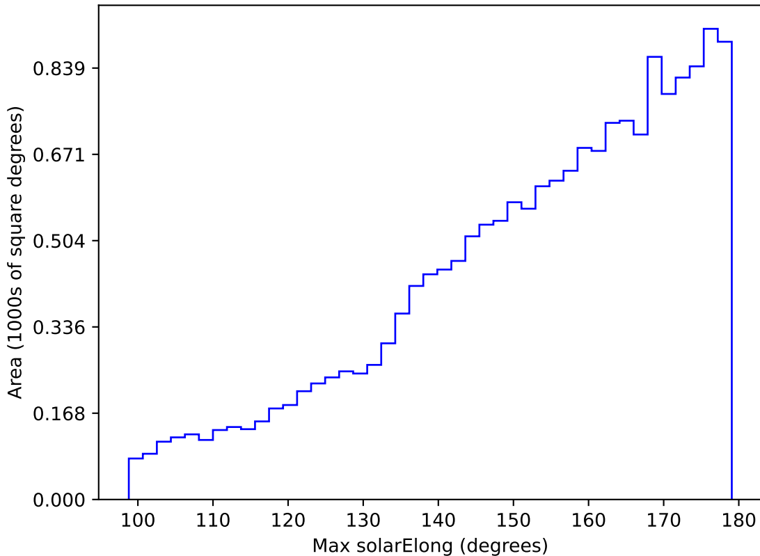
noroll_mjdp365_v3.4_10yrs WFD g band: Max solarElong
