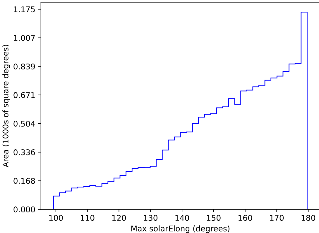
noroll_mjdp365_v3.4_10yrs WFD all bands: Max solarElong
