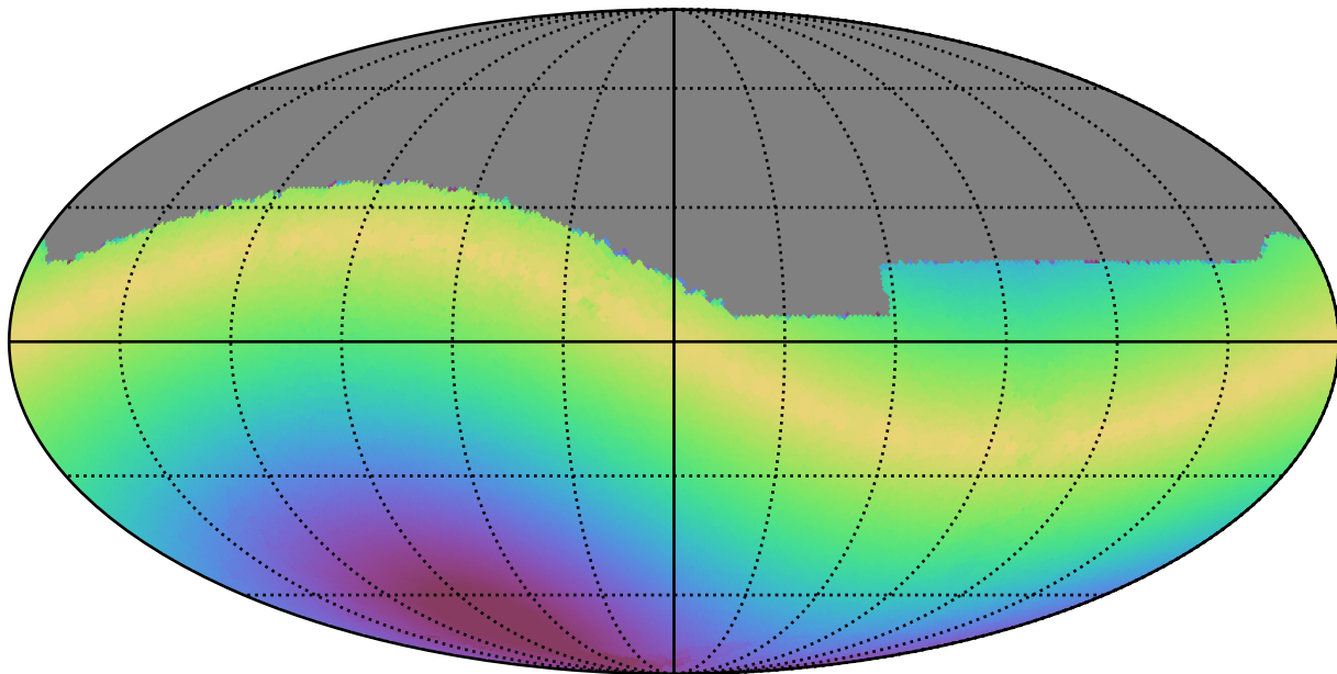
noroll_mjdp365_v3.4_10yrs All sky z band: Max solarElong
