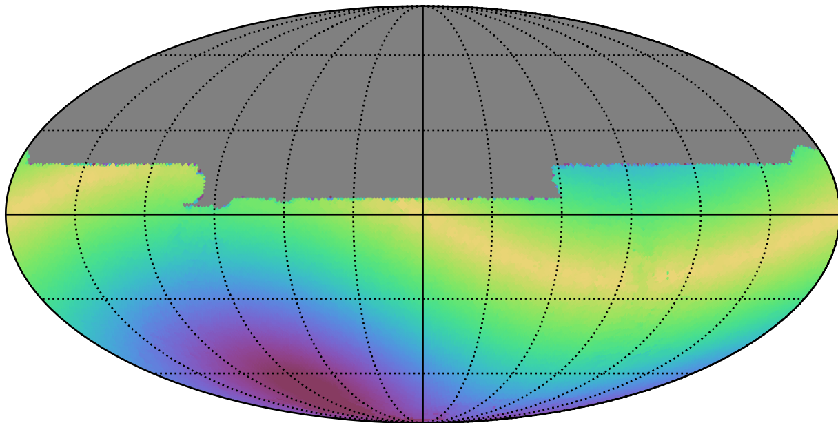
noroll_mjdp365_v3.4_10yrs All sky y band: Max solarElong
