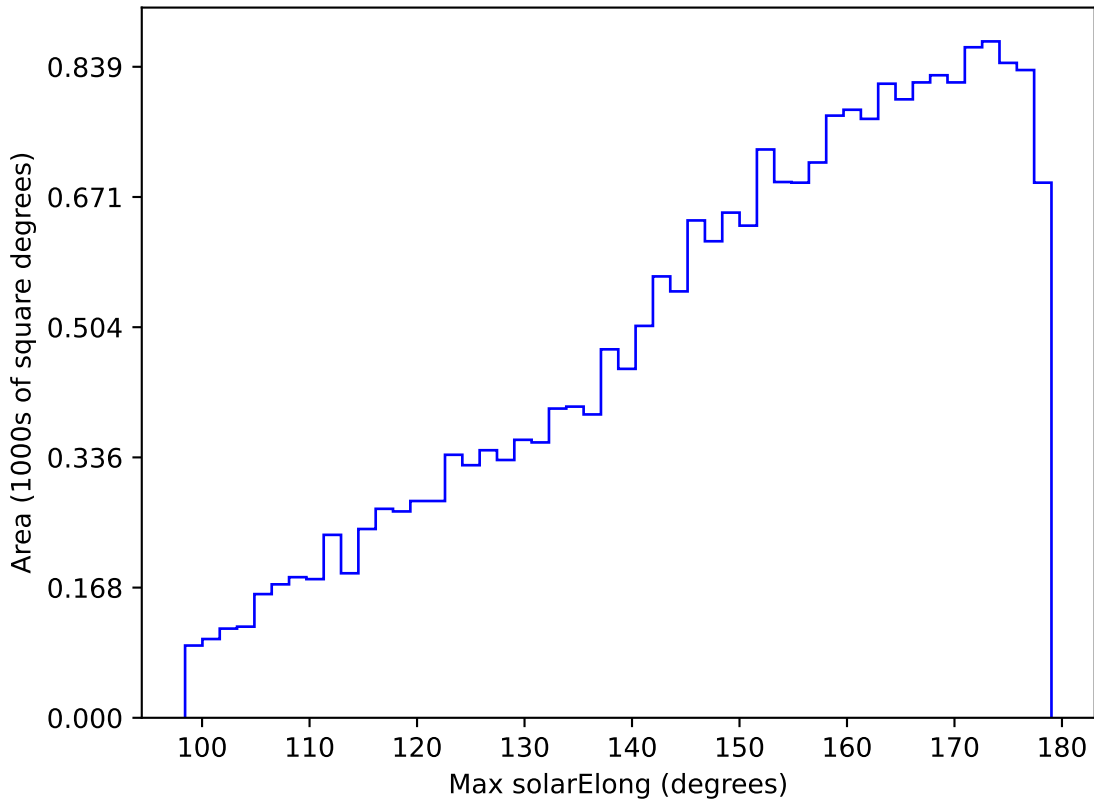
noroll_mjdp365_v3.4_10yrs All sky u band: Max solarElong
