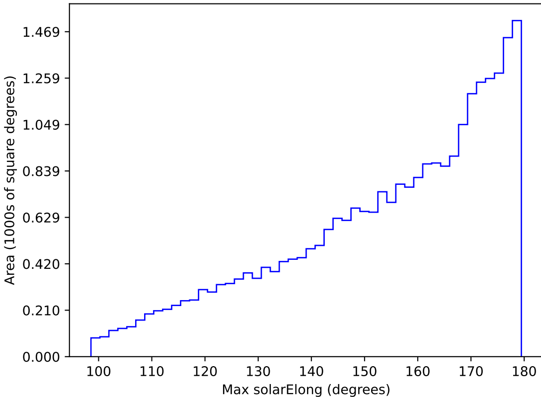
noroll_mjdp365_v3.4_10yrs All sky r band: Max solarElong
