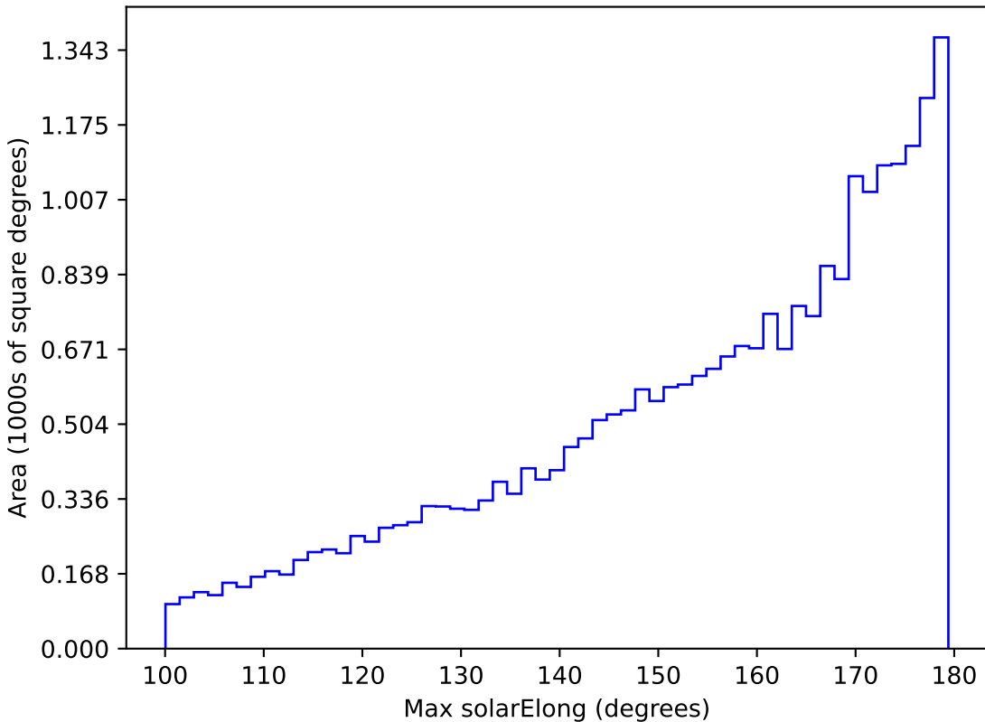
noroll_mjdp365_v3.4_10yrs All sky i band: Max solarElong
