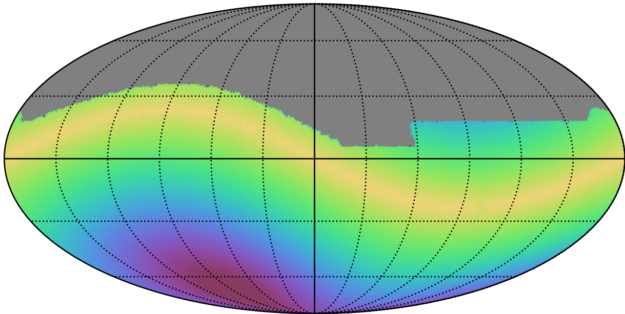
noroll_mjdp365_v3.4_10yrs All sky all bands: Max solarElong
