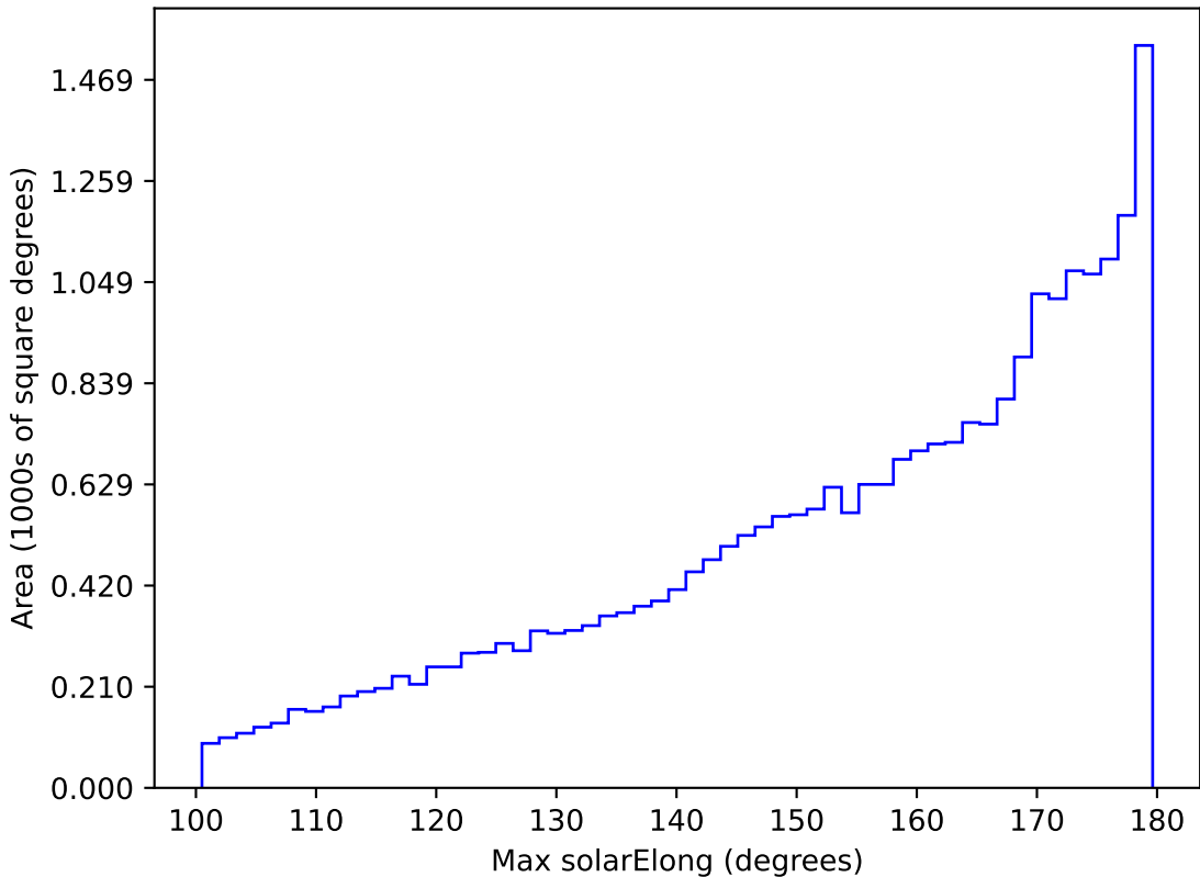
noroll_mjdp365_v3.4_10yrs All sky all bands: Max solarElong
