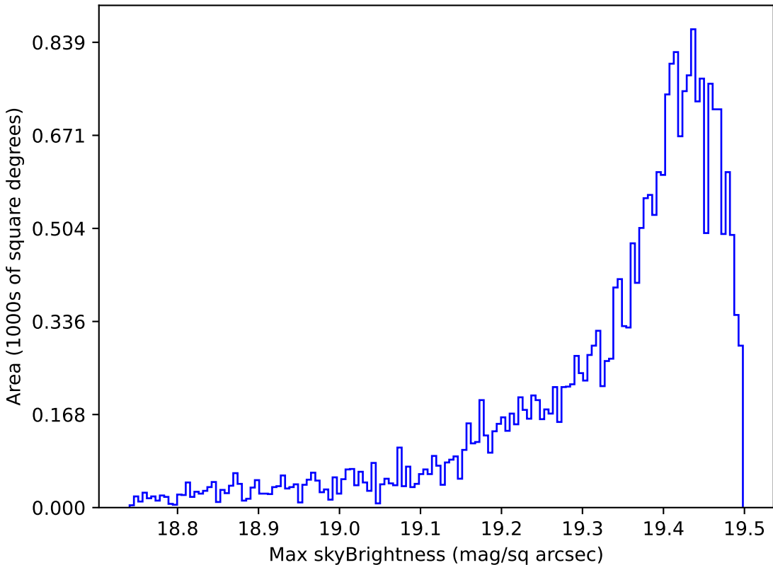
noroll_mjdp365_v3.4_10yrs Yr 1 z band: Max skyBrightness
