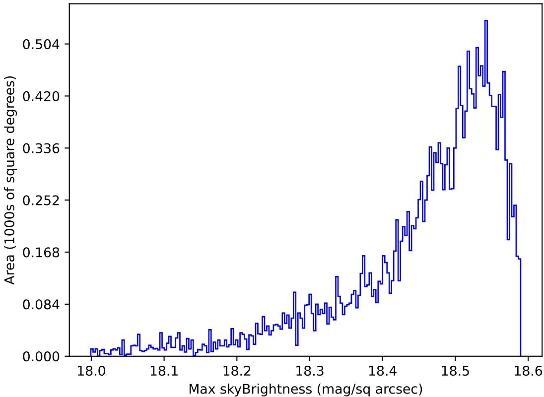
noroll_mjdp365_v3.4_10yrs Yr 1 y band: Max skyBrightness
