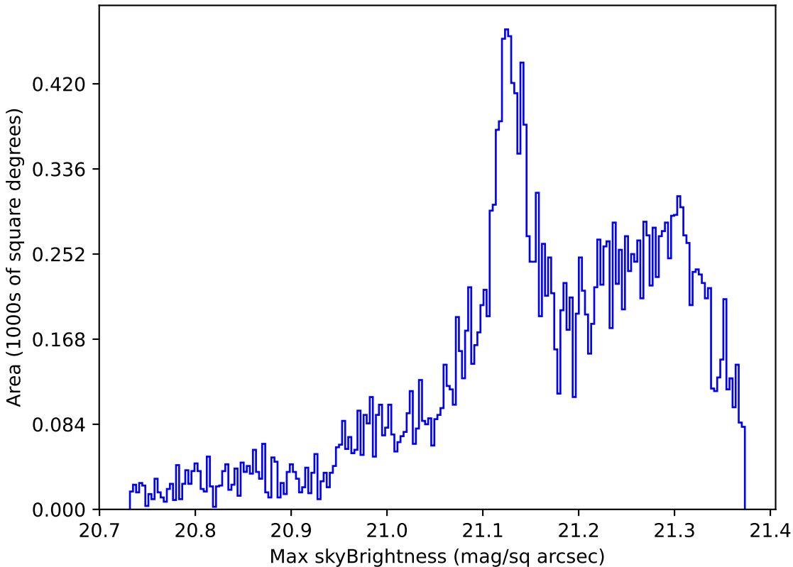
noroll_mjdp365_v3.4_10yrs Yr 1 r band: Max skyBrightness
