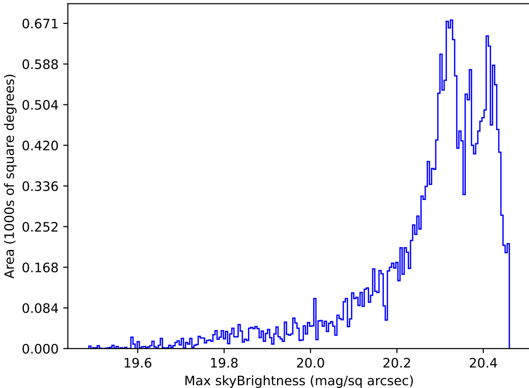
noroll_mjdp365_v3.4_10yrs Yr 1 i band: Max skyBrightness
