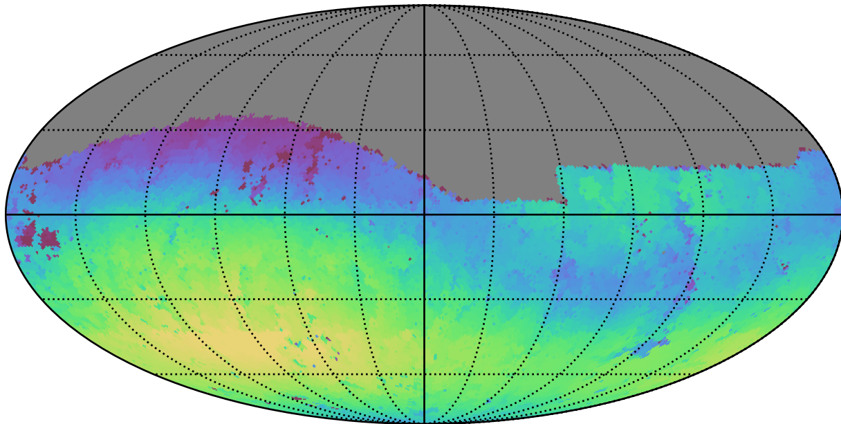
noroll_mjdp365_v3.4_10yrs Yr 1 g band: Max skyBrightness
