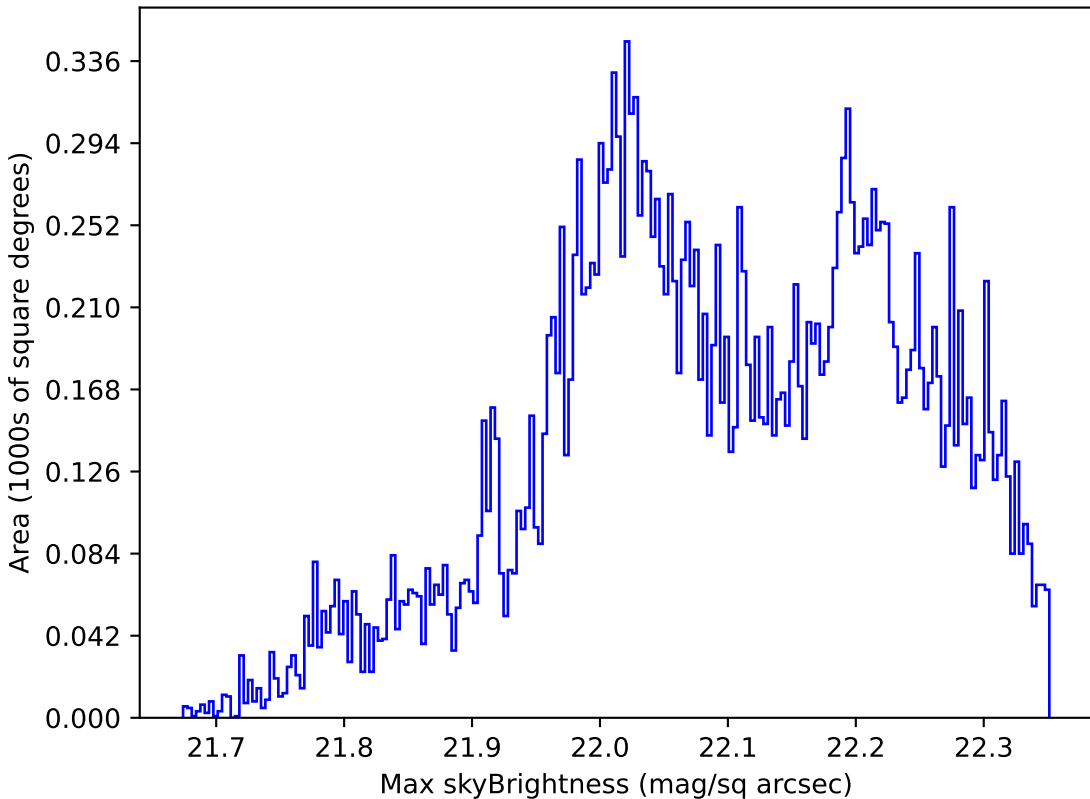
noroll_mjdp365_v3.4_10yrs Yr 1 g band: Max skyBrightness
