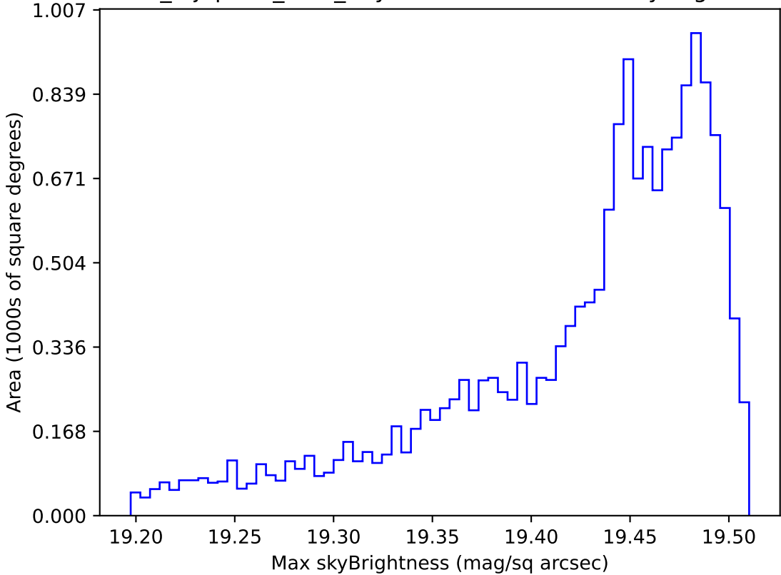
noroll_mjdp365_v3.4_10yrs WFD z band: Max skyBrightness
