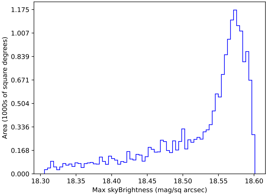
noroll_mjdp365_v3.4_10yrs WFD y band: Max skyBrightness
