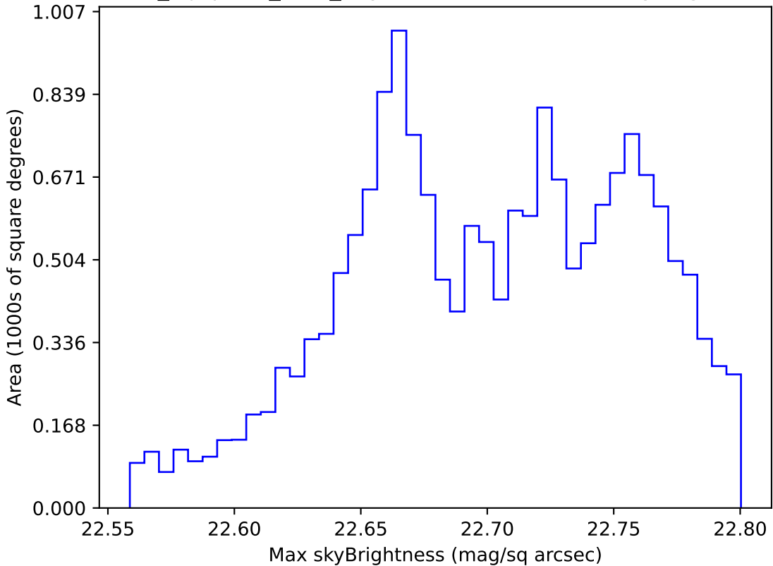
noroll_mjdp365_v3.4_10yrs WFD u band: Max skyBrightness
