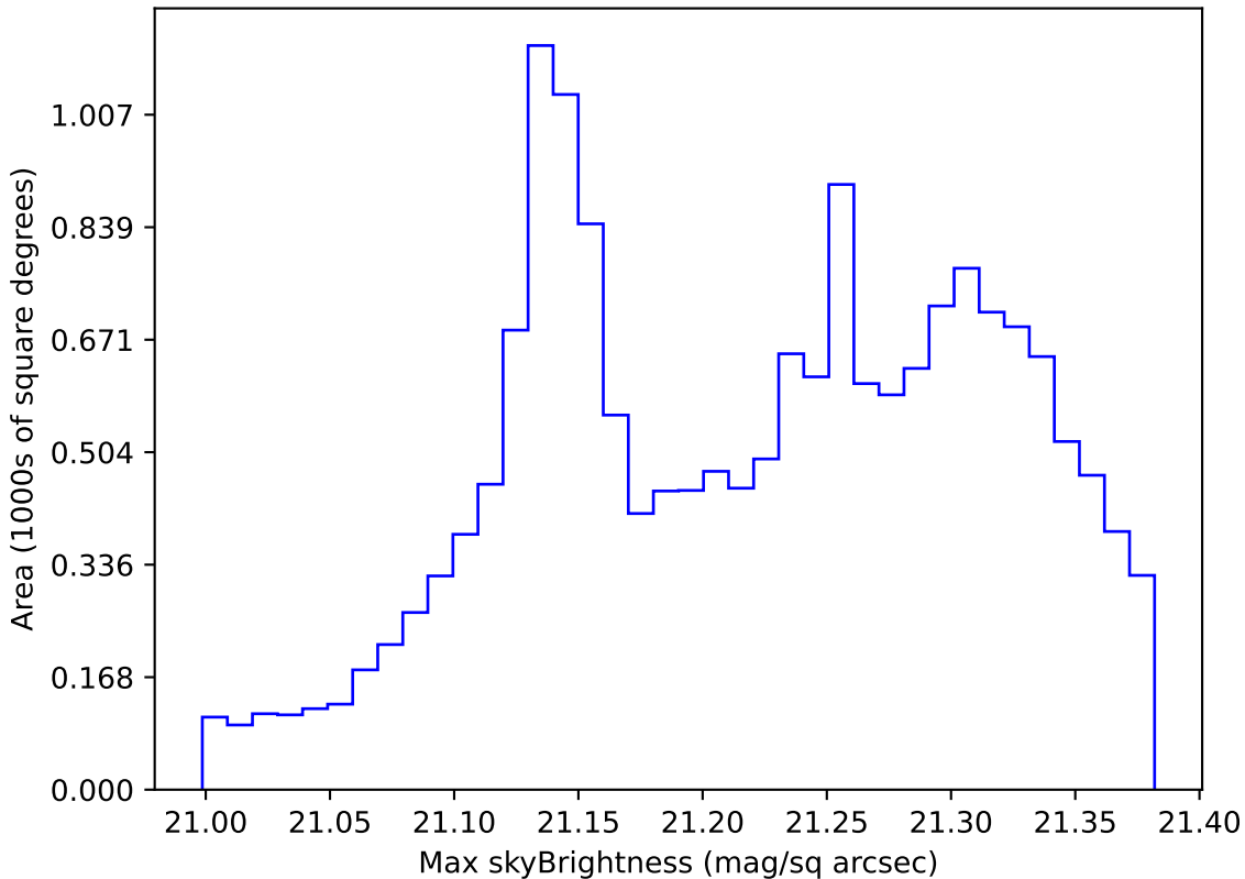
noroll_mjdp365_v3.4_10yrs WFD r band: Max skyBrightness
