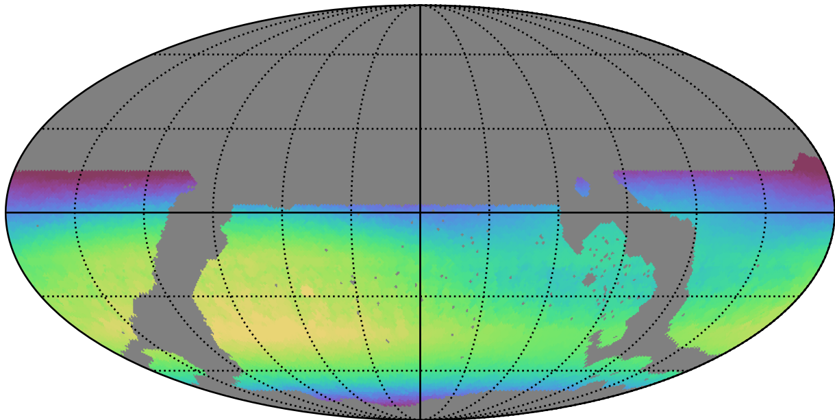
noroll_mjdp365_v3.4_10yrs WFD i band: Max skyBrightness
