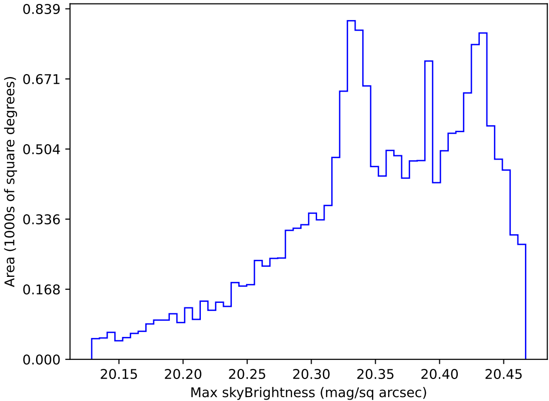
noroll_mjdp365_v3.4_10yrs WFD i band: Max skyBrightness
