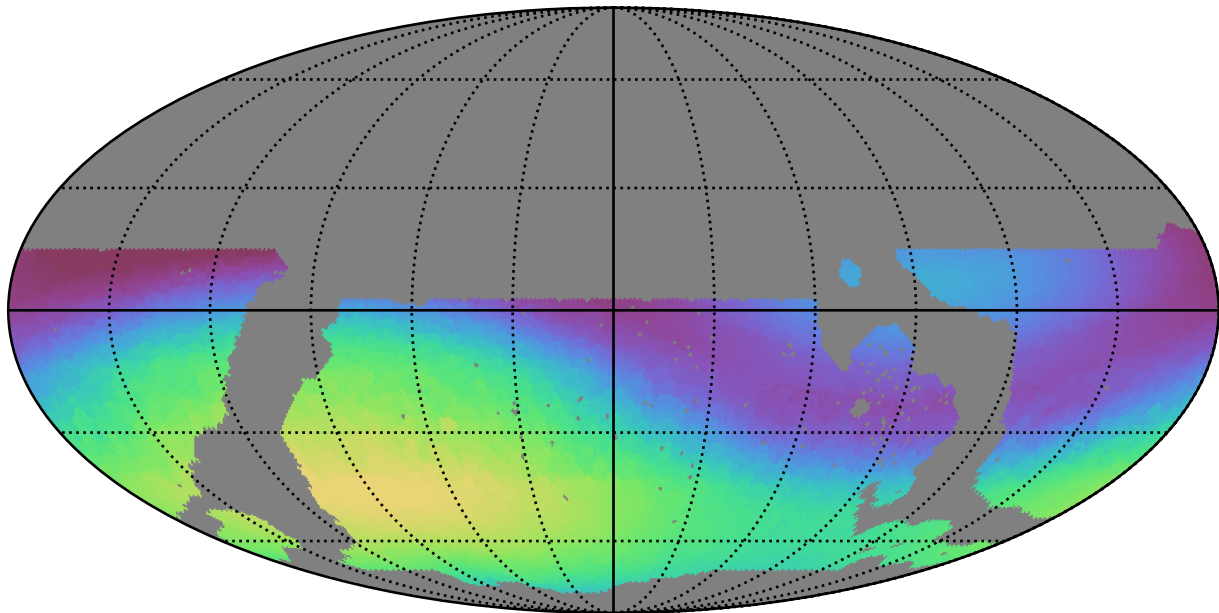
noroll_mjdp365_v3.4_10yrs WFD g band: Max skyBrightness
