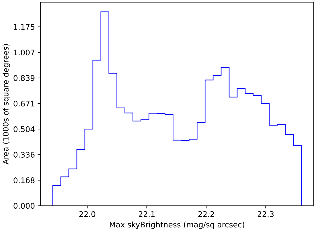
noroll_mjdp365_v3.4_10yrs WFD g band: Max skyBrightness
