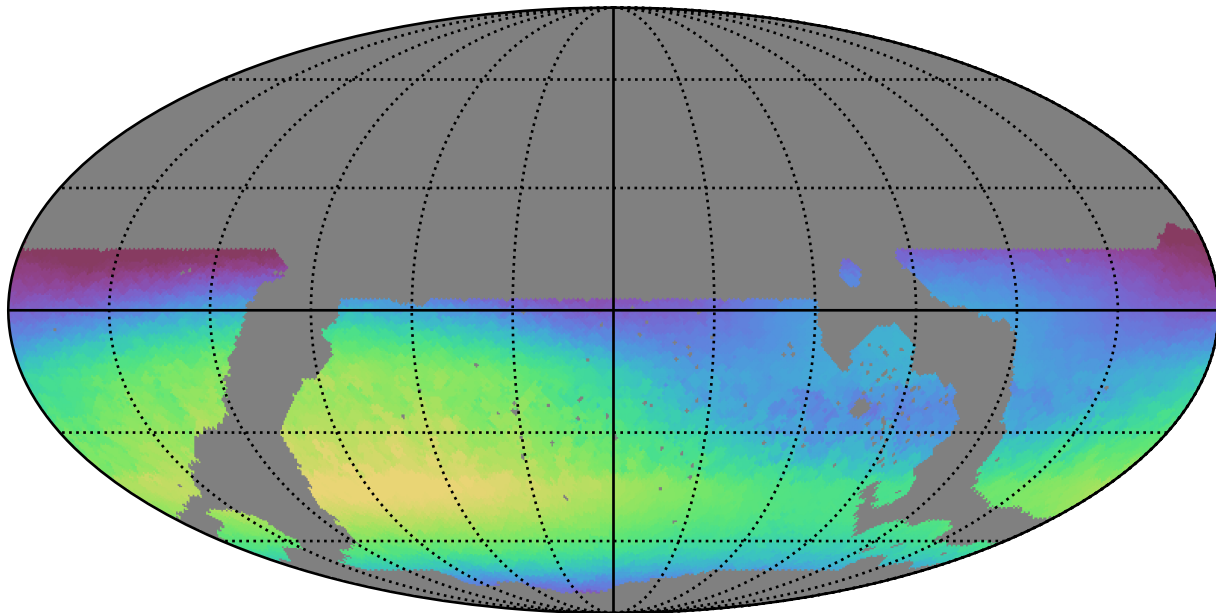
noroll_mjdp365_v3.4_10yrs WFD all bands: Max skyBrightness
