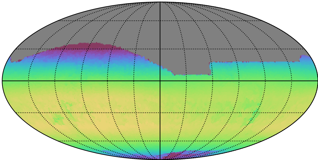
noroll_mjdp365_v3.4_10yrs All sky z band: Max skyBrightness
