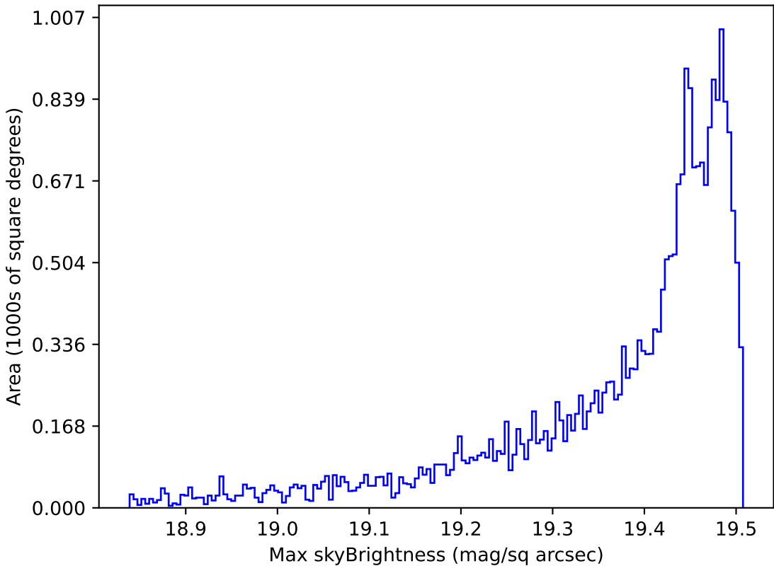
noroll_mjdp365_v3.4_10yrs All sky z band: Max skyBrightness
