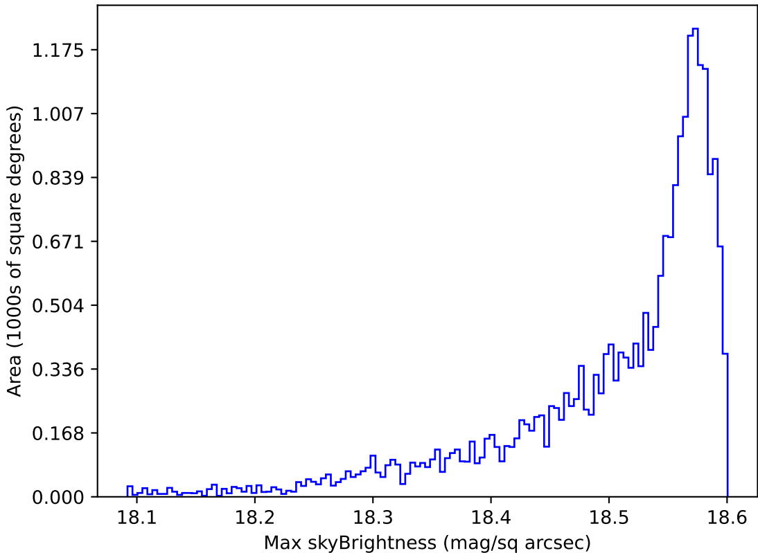
noroll_mjdp365_v3.4_10yrs All sky y band: Max skyBrightness
