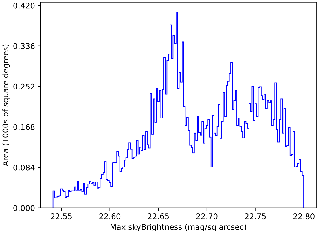
noroll_mjdp365_v3.4_10yrs All sky u band: Max skyBrightness
