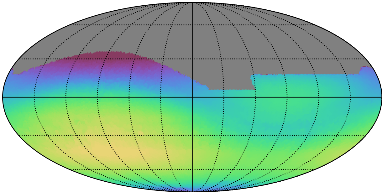
noroll_mjdp365_v3.4_10yrs All sky r band: Max skyBrightness
