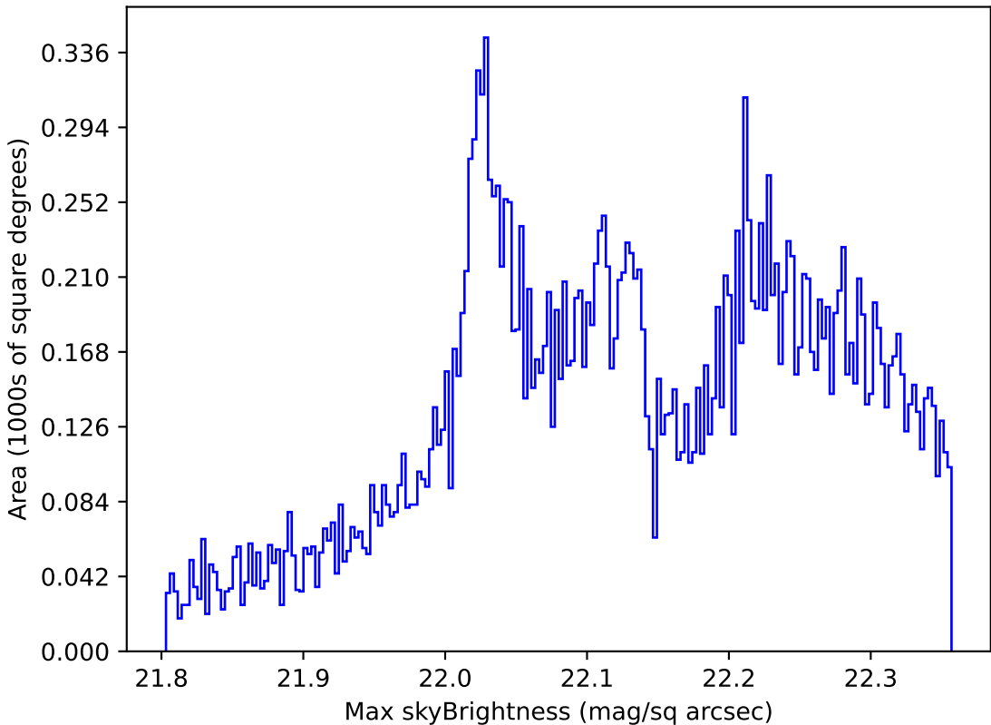
noroll_mjdp365_v3.4_10yrs All sky g band: Max skyBrightness
