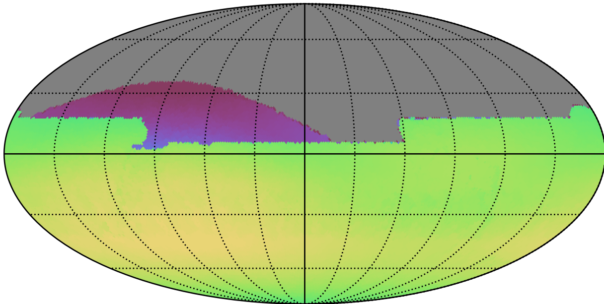
noroll_mjdp365_v3.4_10yrs All sky all bands: Max skyBrightness
