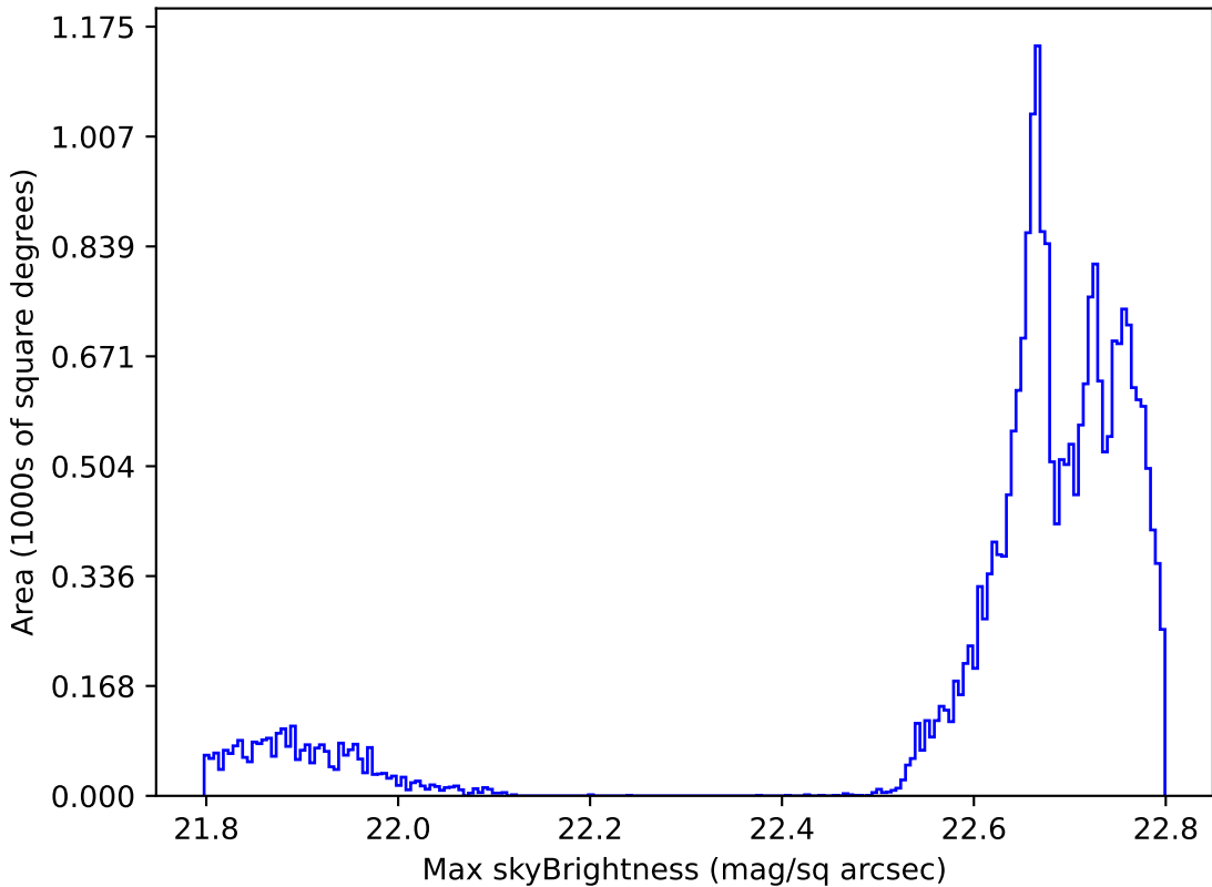
noroll_mjdp365_v3.4_10yrs All sky all bands: Max skyBrightness
