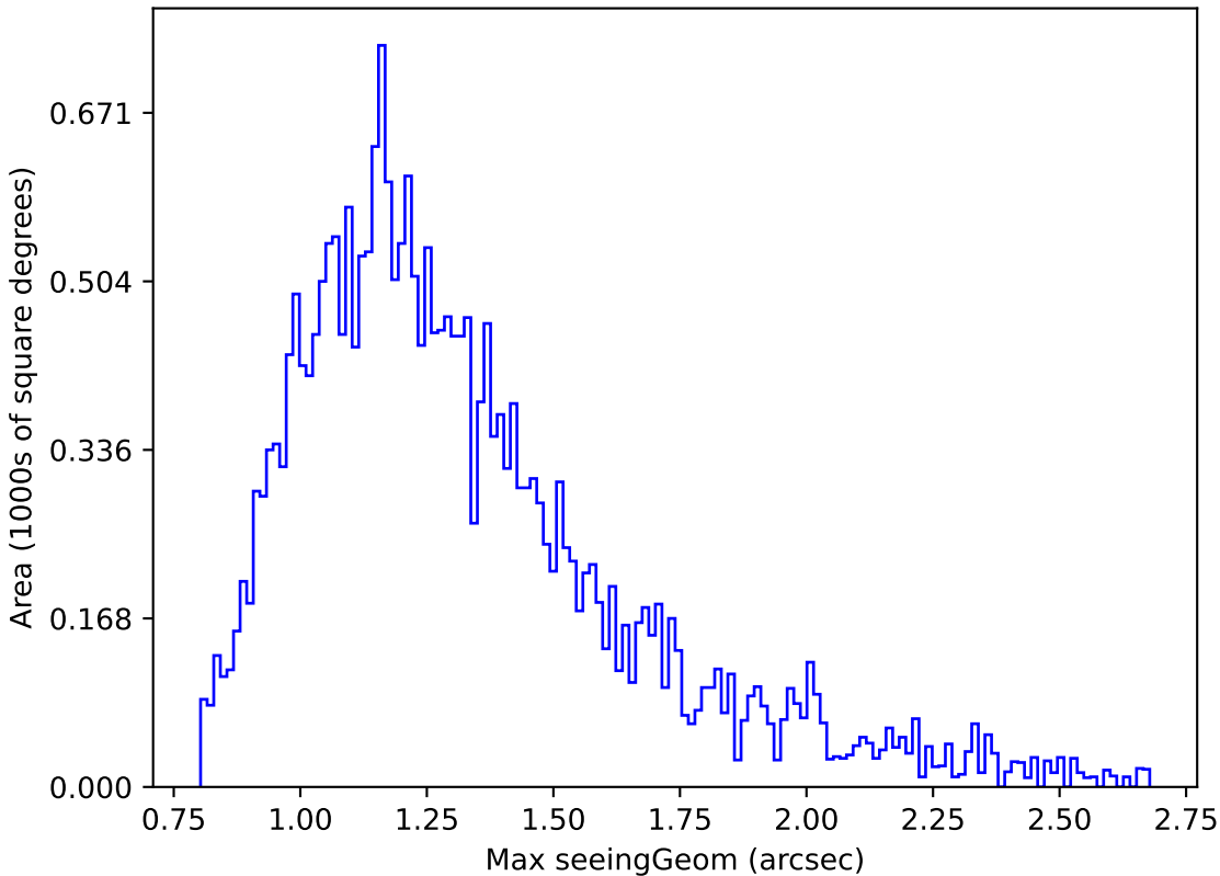
noroll_mjdp365_v3.4_10yrs Yr 1 z band: Max seeingGeom
