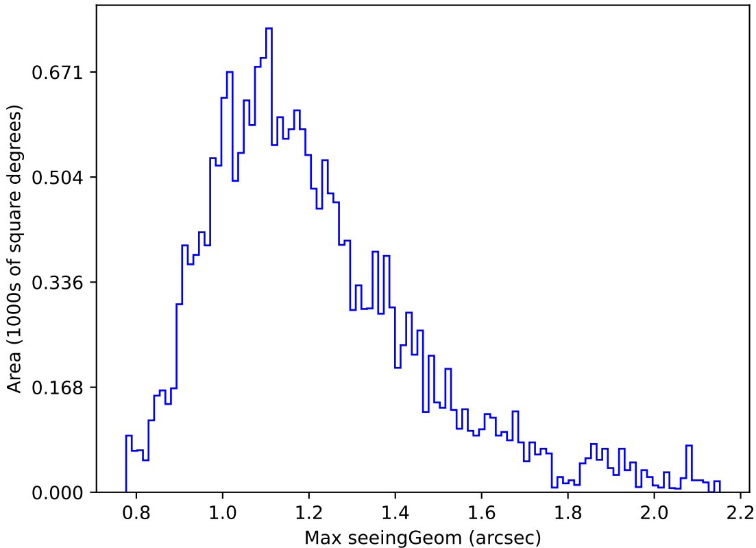
noroll_mjdp365_v3.4_10yrs Yr 1 y band: Max seeingGeom
