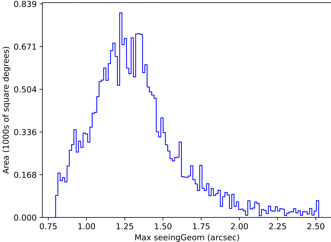
noroll_mjdp365_v3.4_10yrs Yr 1 i band: Max seeingGeom
