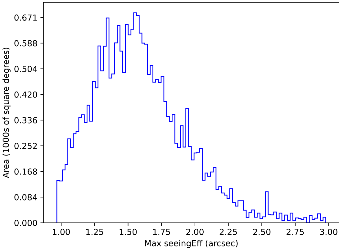
noroll_mjdp365_v3.4_10yrs Yr 1 u band: Max seeingEff
