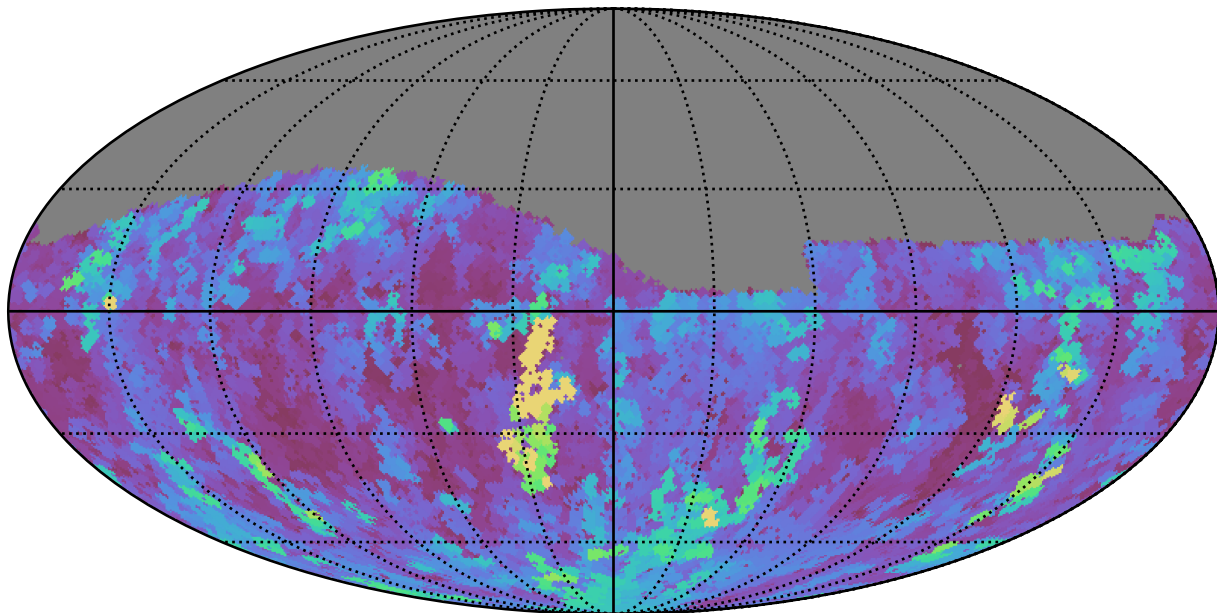
noroll_mjdp365_v3.4_10yrs Yr 1 g band: Max seeingEff
