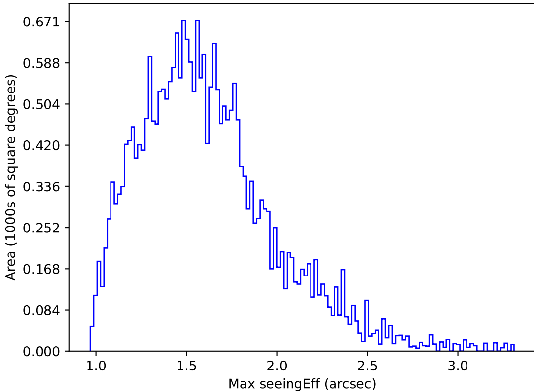
noroll_mjdp365_v3.4_10yrs Yr 1 g band: Max seeingEff
