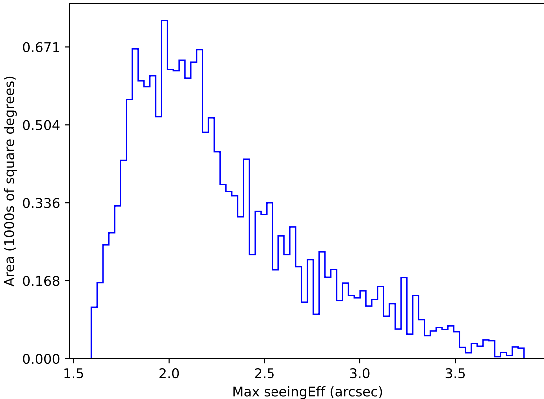
noroll_mjdp365_v3.4_10yrs WFD y band: Max seeingEff
