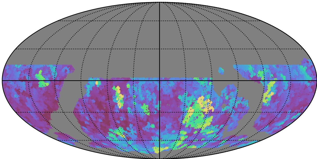
noroll_mjdp365_v3.4_10yrs WFD i band: Max seeingEff
